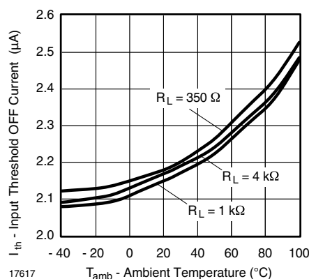
Figure 9. Input Threshold OFF Current vs. Ambient Temperature
