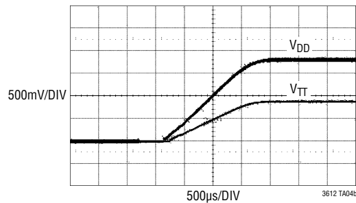
Ratiometric Start-Up
