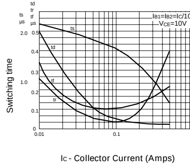
Switching Speeds
