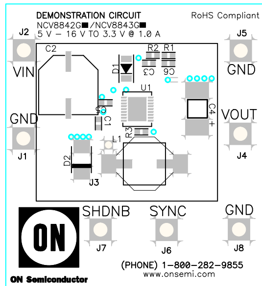
Figure 17. Top Silk
