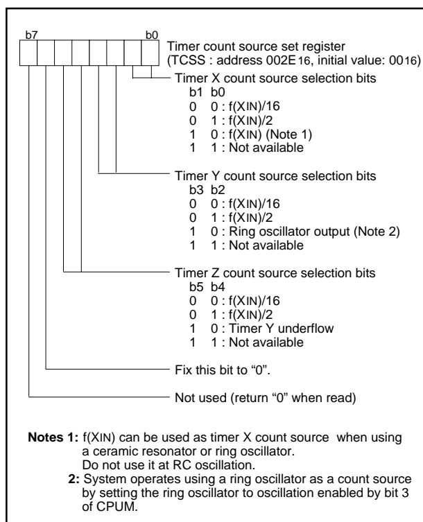
Fig. 24 Timer count source set register
