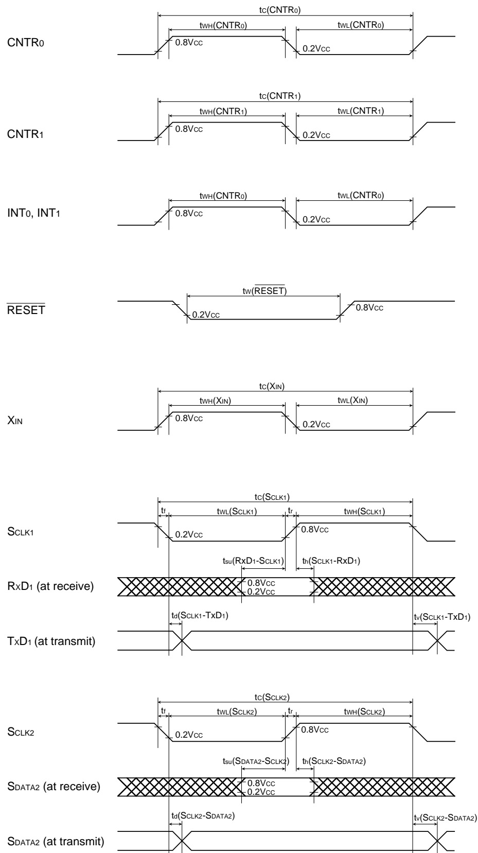
Fig. 57 Timing chart (Extended operating temperature 125 °C version)
