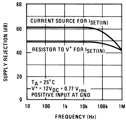
Supply Rejection
