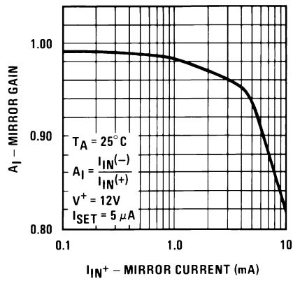
Mirror Gain
