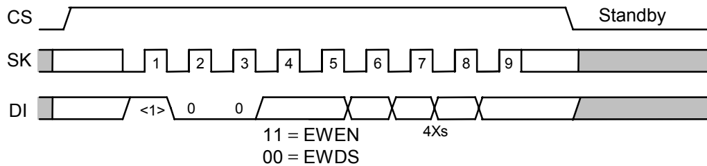
Figure 17 Write Enable/Disable Timing (S-93C46B)
