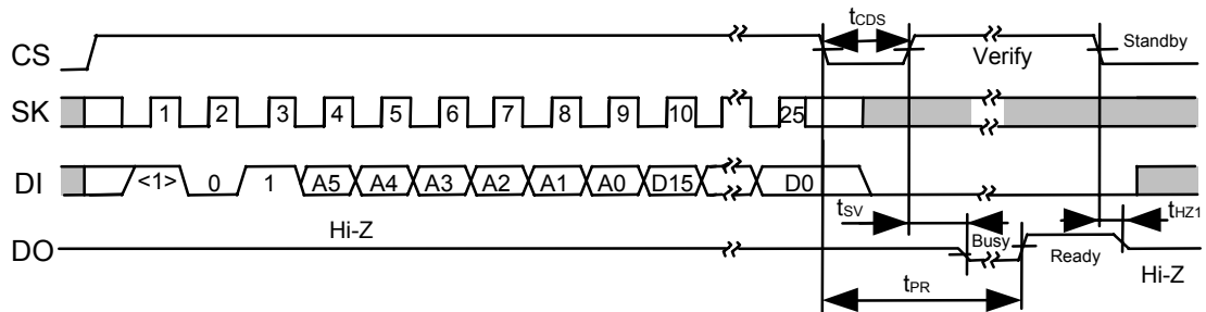
Figure 9 Data Write Timing (S-93C46B)
