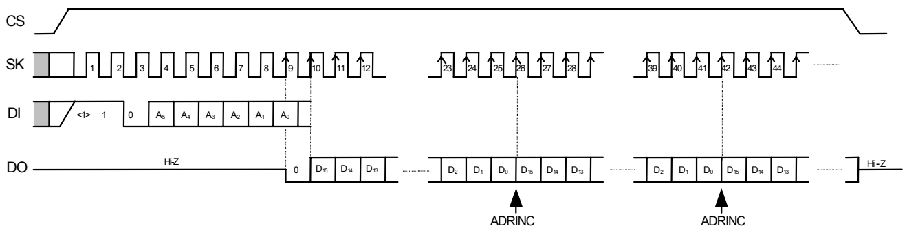
Figure 7 Read Timing (S-93C46B)
