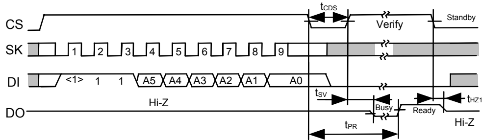
Figure 11 Data Erase Timing (S-93C46B)
