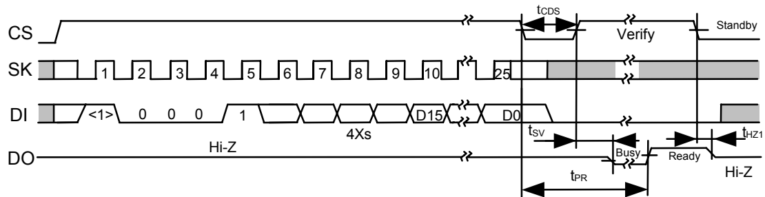
Figure 13 Chip Write Timing (S-93C46B)
