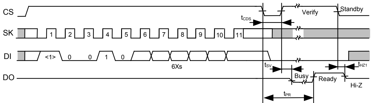
Figure 16 Chip Erase Timing (S-93C56B, S-93C66B)
