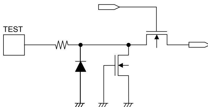
Figure 24 TEST Pin
