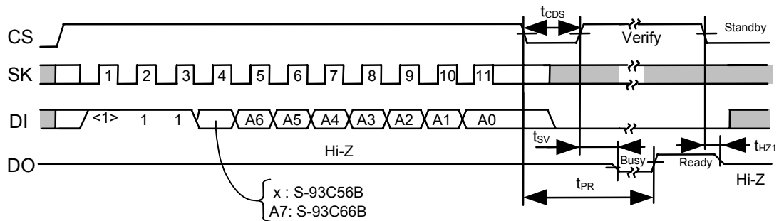
Figure 12 Data Erase Timing (S-93C56B, S-93C66B)
