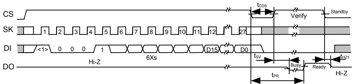
Figure 13 Chip Write Timing (S-93C46B)
