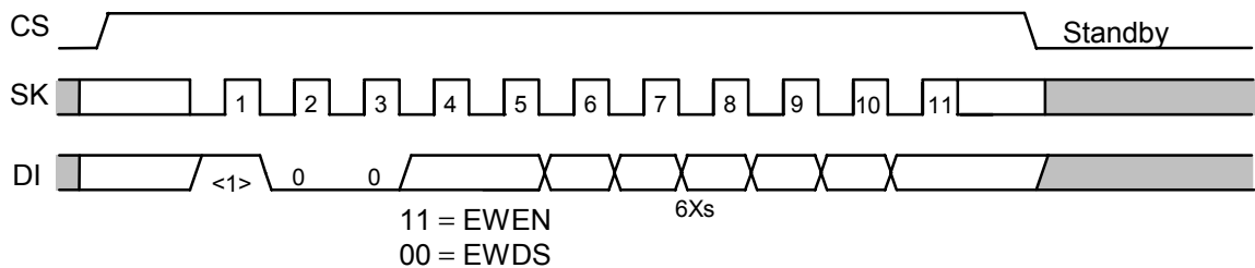
Figure 18 Write Enable/Disable Timing (S-93C56B, S-93C66B)
