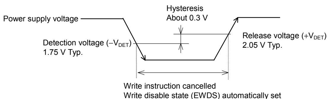
Figure 19 Operation when Power Supply Voltage is Low
