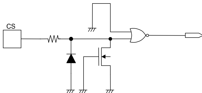
Figure 22 CS Pin
