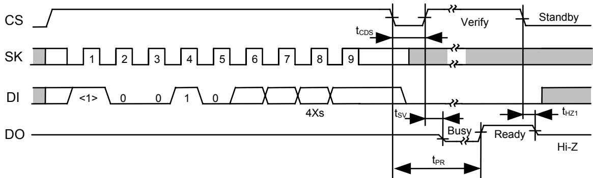
Figure 15 Chip Erase Timing (S-93C46B)
