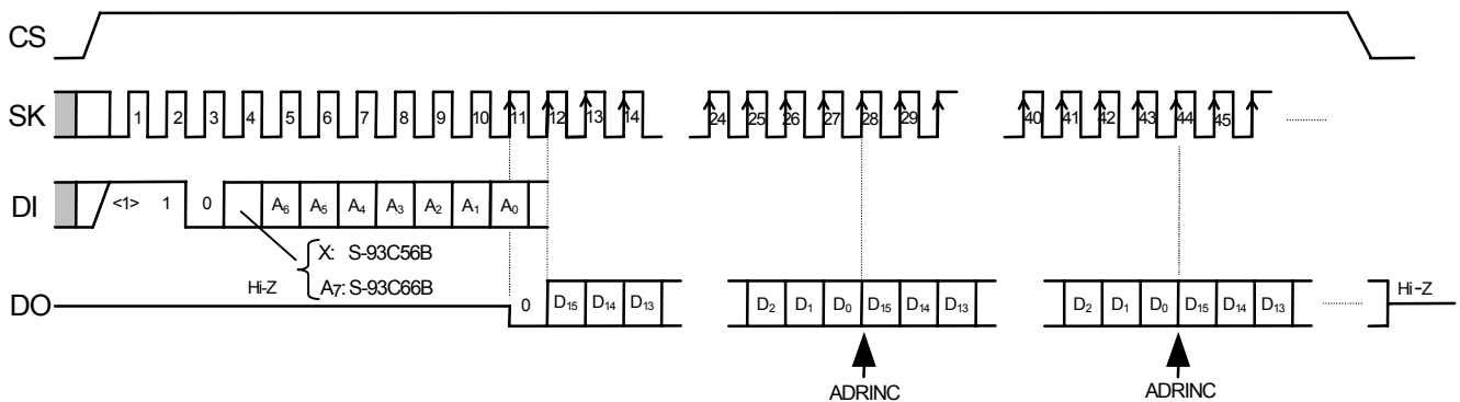
Figure 8 Read Timing (S-93C56B, S-93C66B)
