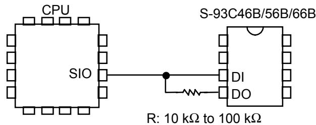
Figure 21 Connection of 3-Wire Interface
