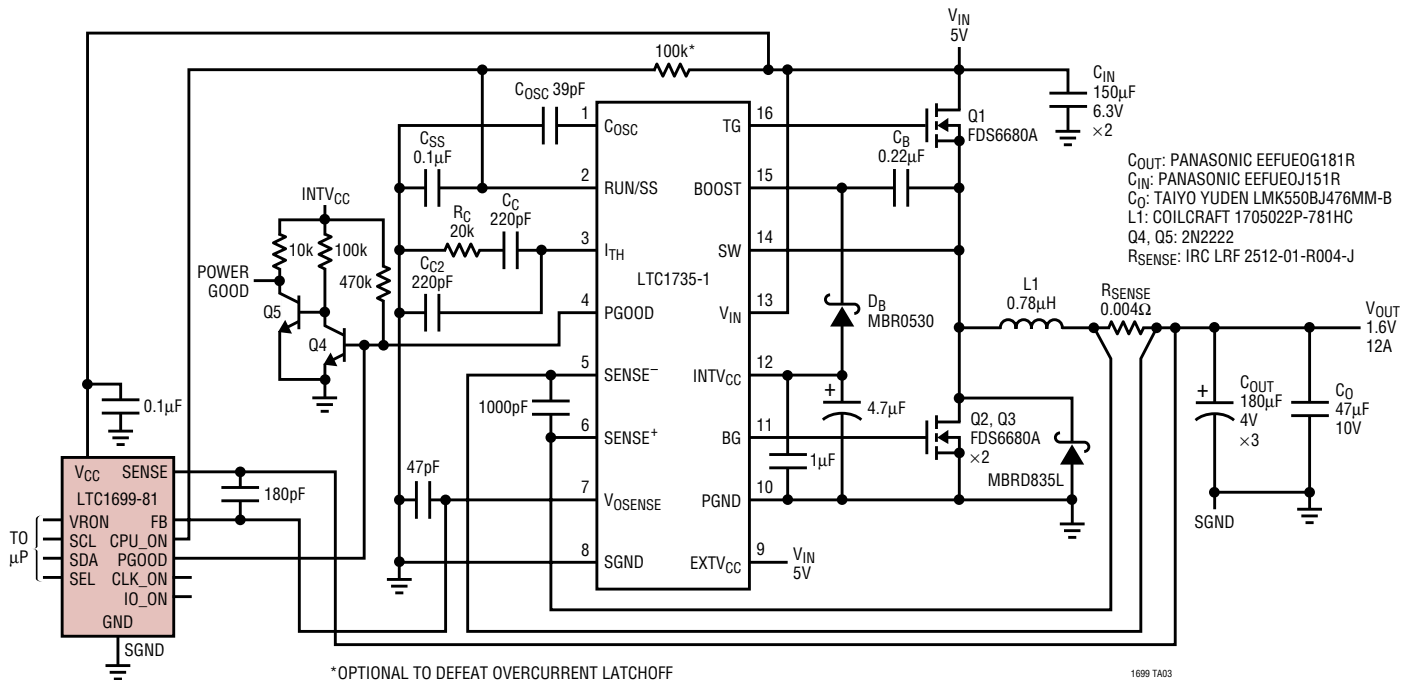
SMBus Programmed CPU Core Voltage Regulator for 2-Step Applications ( V_{IN} = 5V ) with Burst Mode Operation Disabled
