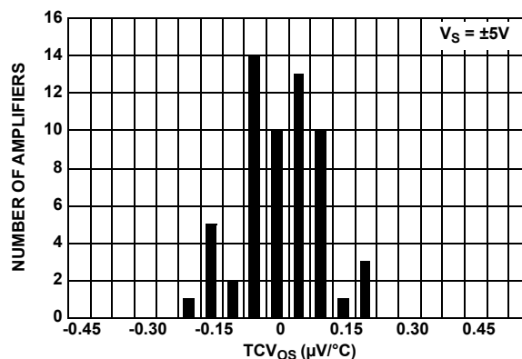
FIGURE 8. TCV_{OS} vs NUMBER OF AMPLIFIERS, V_S = \pm 5V
