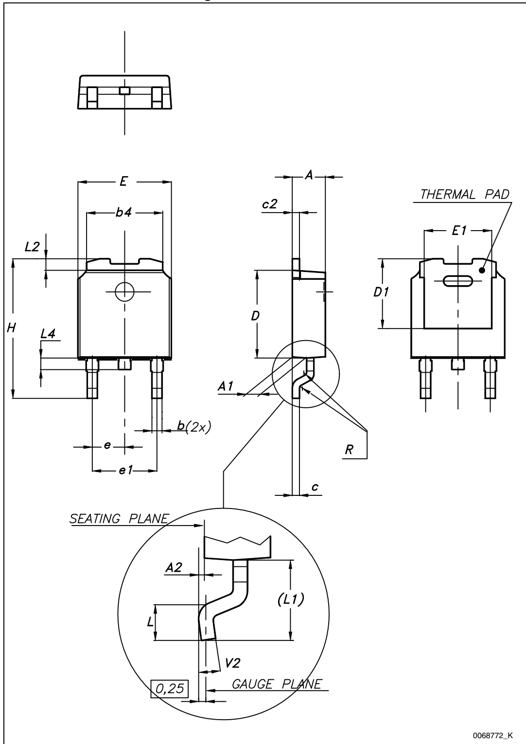
Figure 23. DPAK outline
