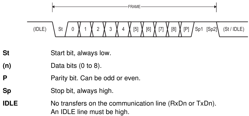
Figure 17-4. Frame Formats
