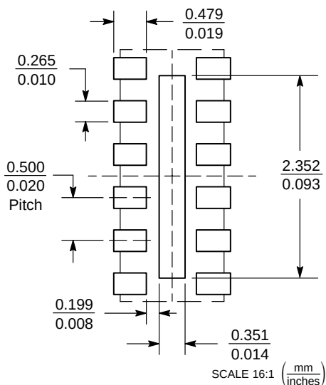
SOLDERING FOOTPRINT*
