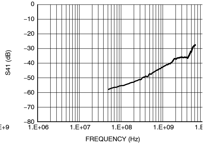
Figure 5. Typical Analog Crosstalk
