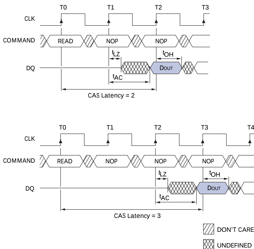
Figure 6: CAS Latency Diagram
