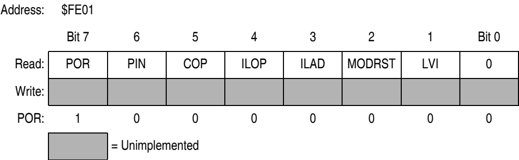
Figure 7-21. Reset Status Register (RSR)
