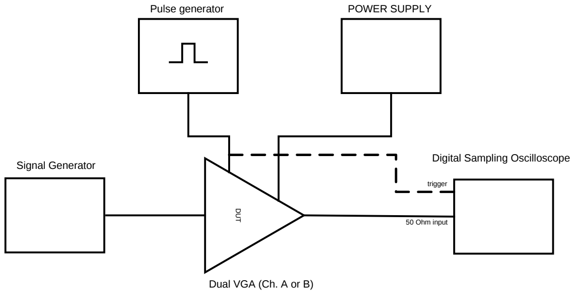
Fig. 10 Timing measurements
