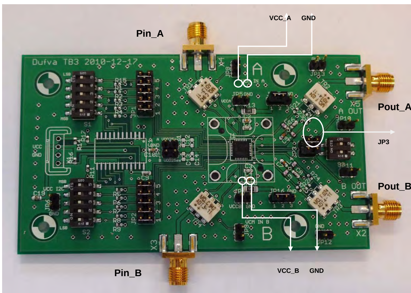
Fig 4. BGA7350 EVB picture
