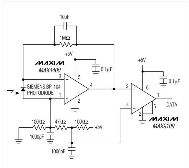
Figure 3. Battery-Operated Infrared Data Link Consumes Only 760 \mu A
