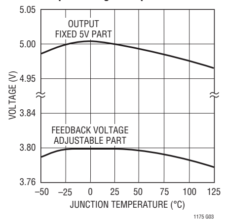
Output Voltage Temperature Drift
