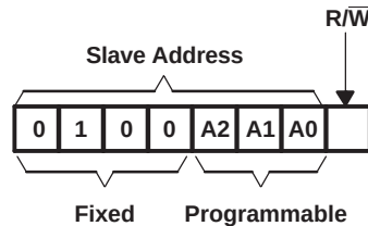
Figure 22. Pca9535 Address
