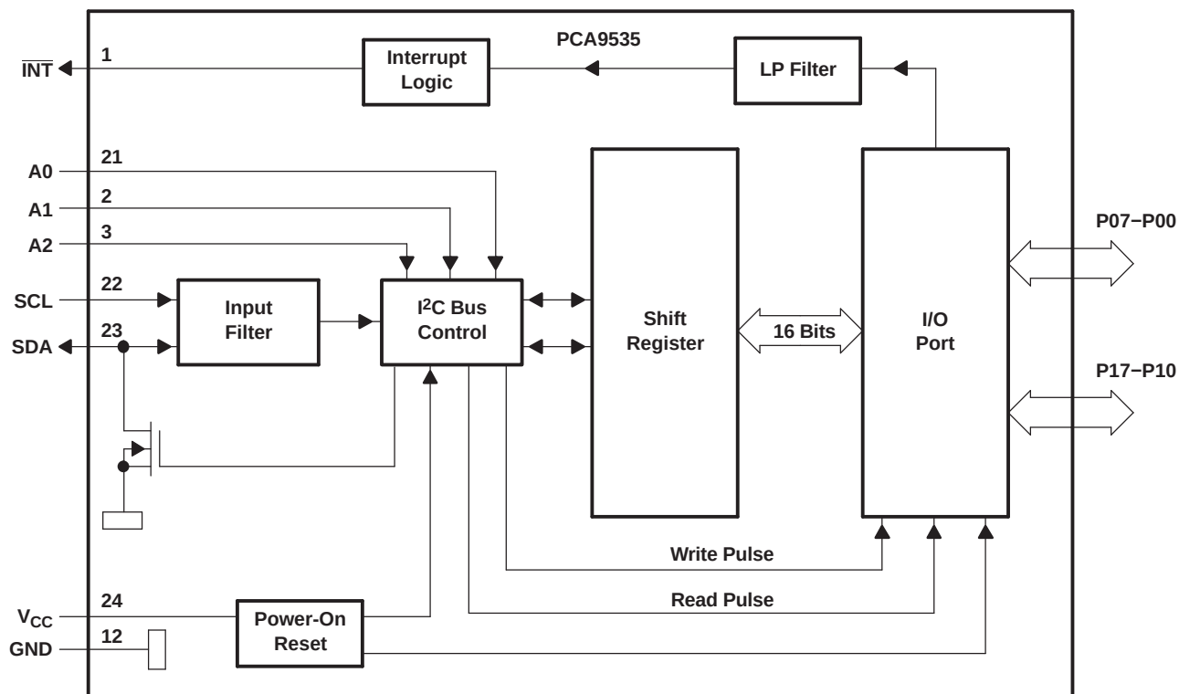
Figure 16. Logic Diagram (Positive Logic)
