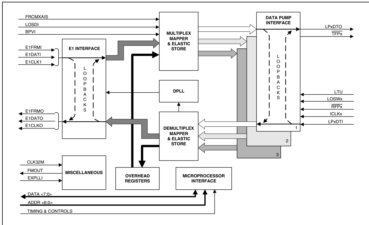
Figure 1. LXP710 Block Diagram
