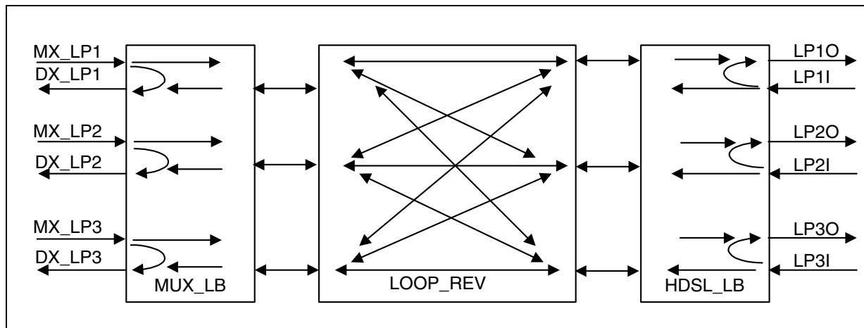
Figure 6. HDSL Interface
