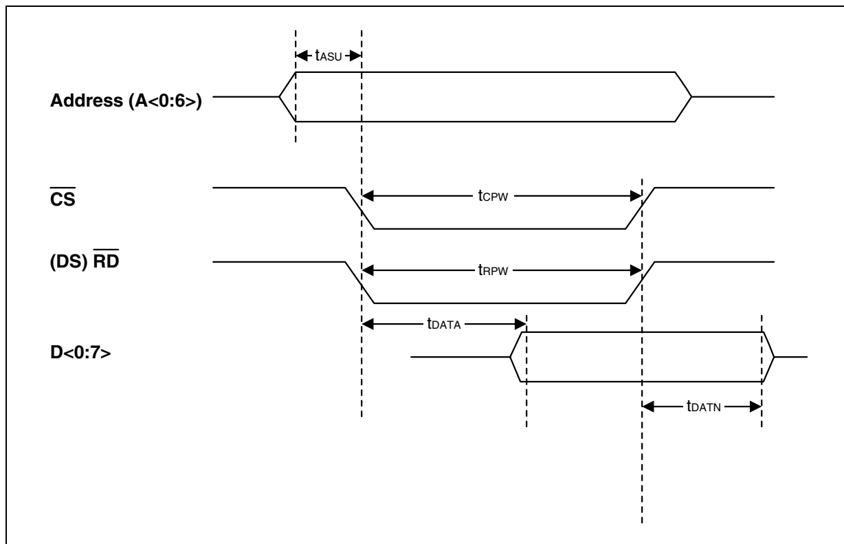
Figure 18. Microprocessor Read Cycle—Intel Mode
