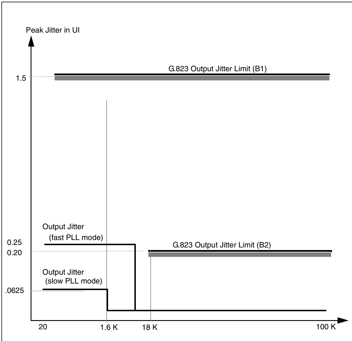
Figure 19. Peak Output Jitter Performance
