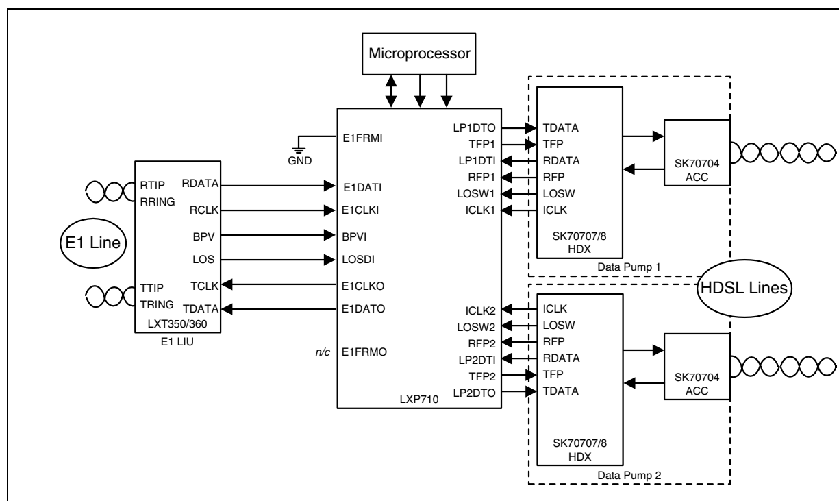
Figure 8. Unframed Data Transport Operation
