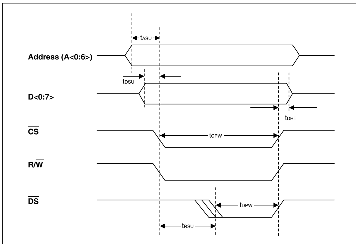
Figure 15. Microprocessor Write Cycle—Motorola Mode
