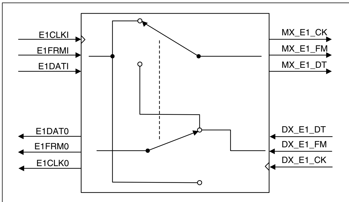
Figure 5. E1 Interface with Loopback Switching
