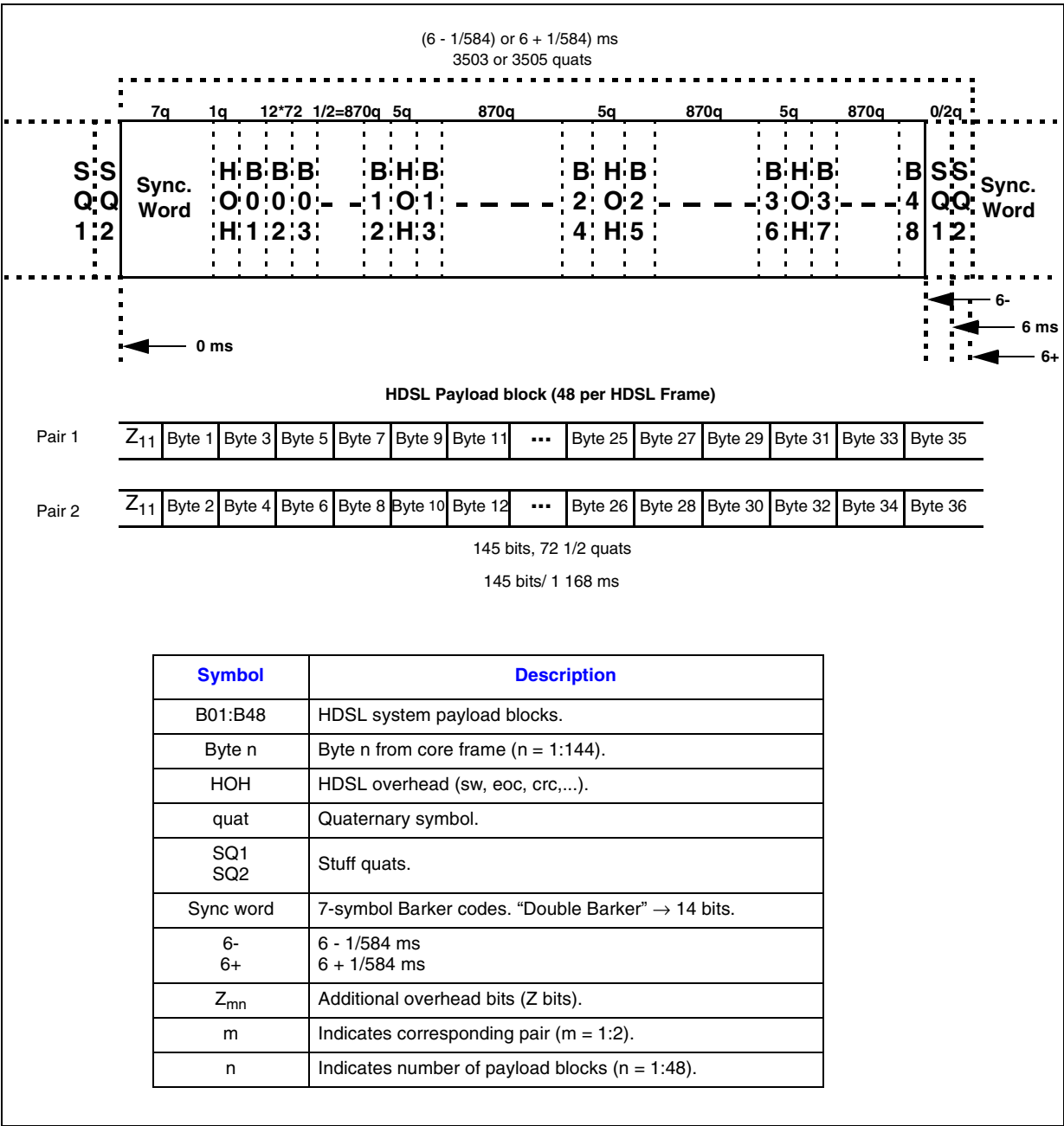
Figure 10. Frame Structure of Two Pair Point-to-Point System
