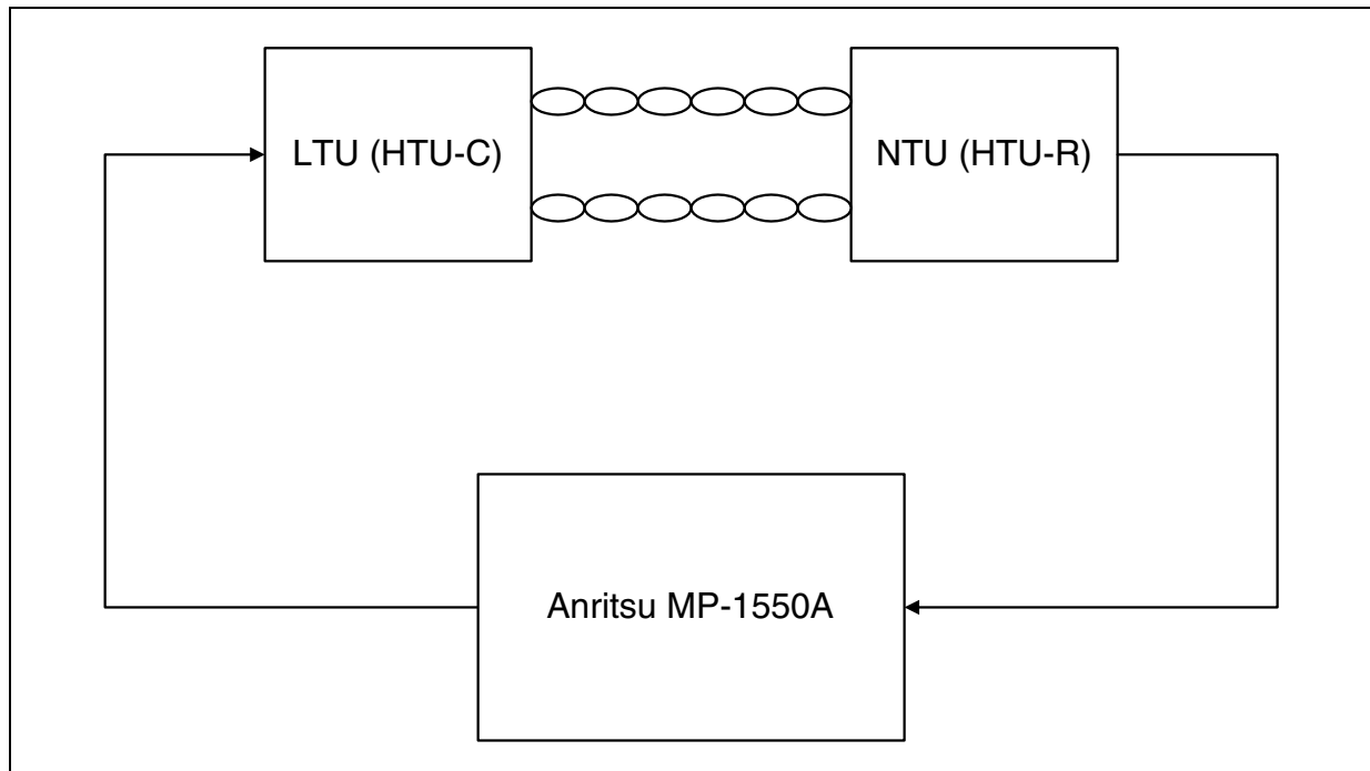
Figure 22. Jitter Transfer Measurement Setup
