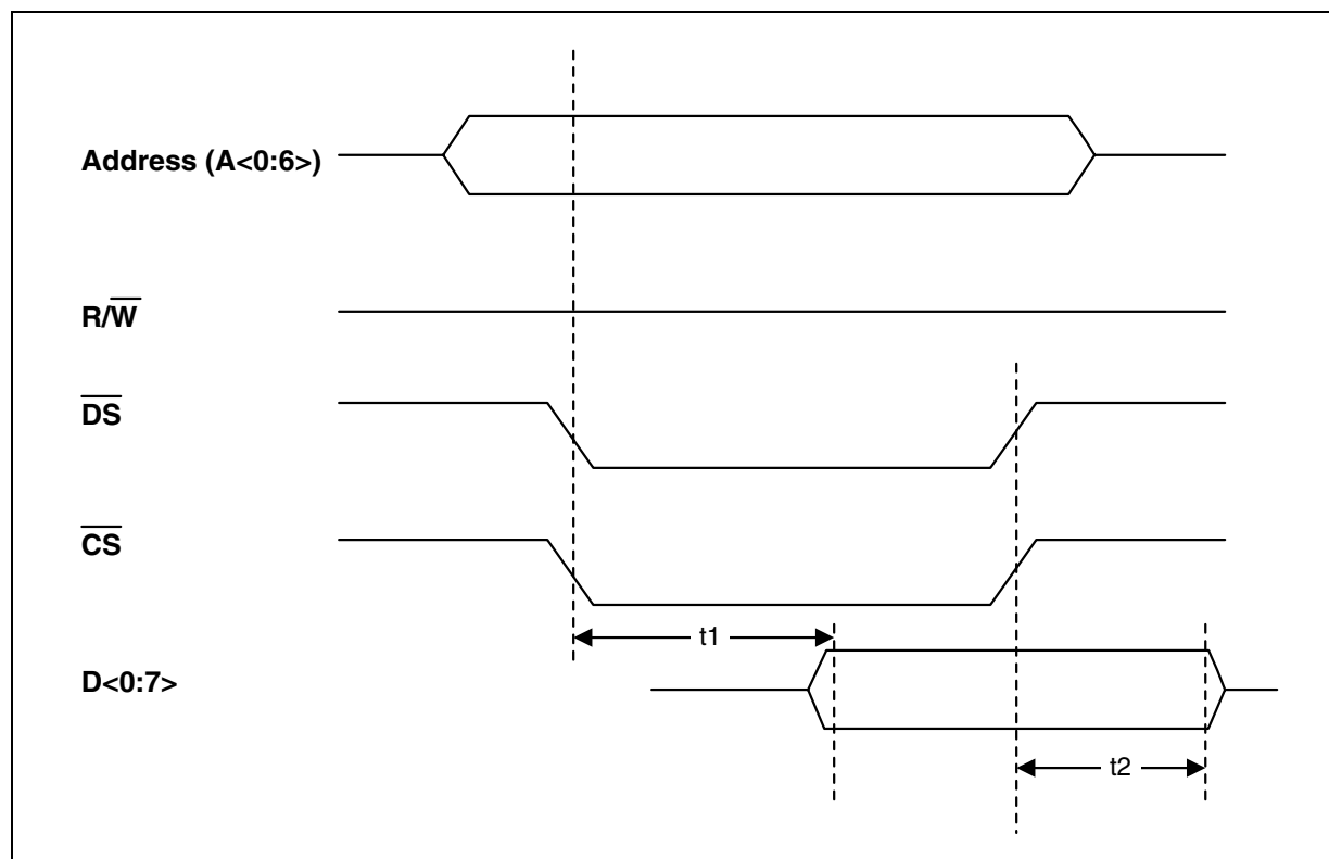
Figure 16. Microprocessor Read Cycle—Motorola Mode
