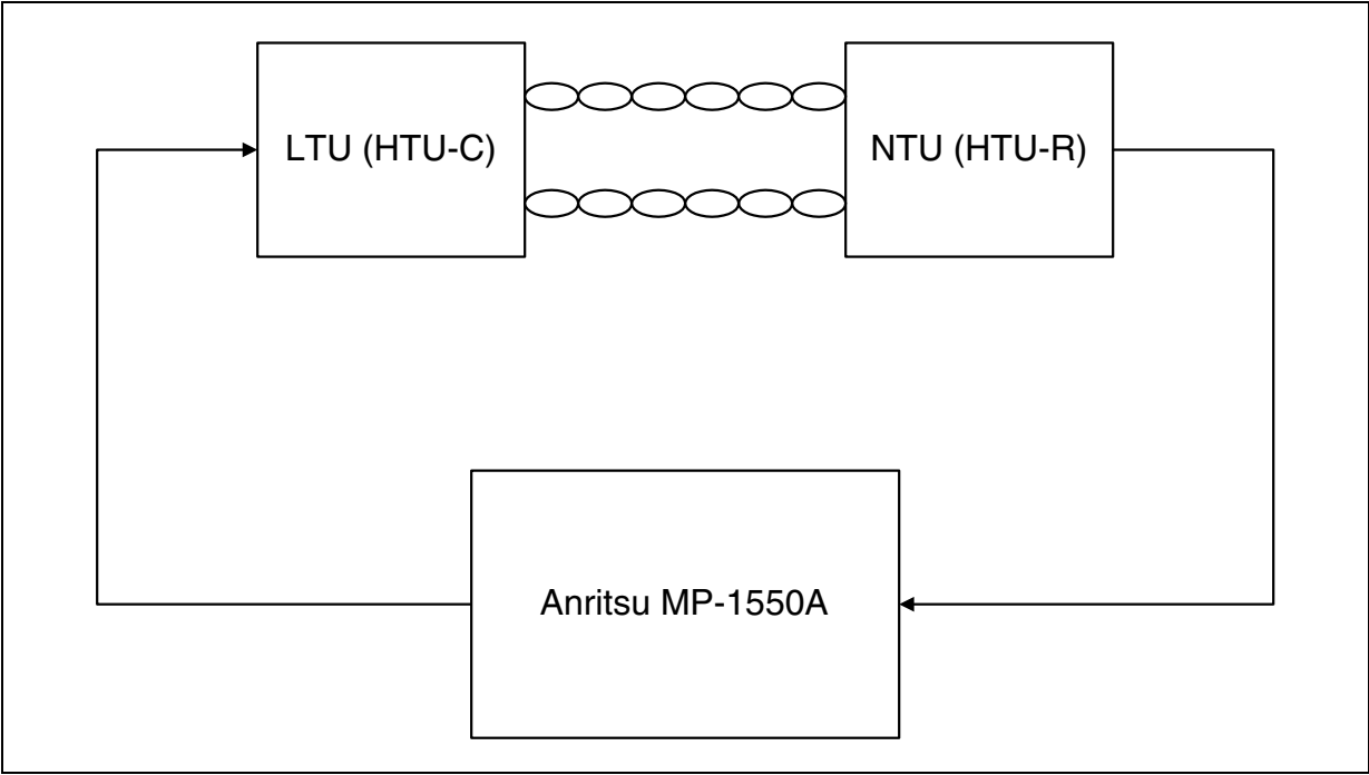
Figure 24. Jitter Tolerance Measurement Setup
