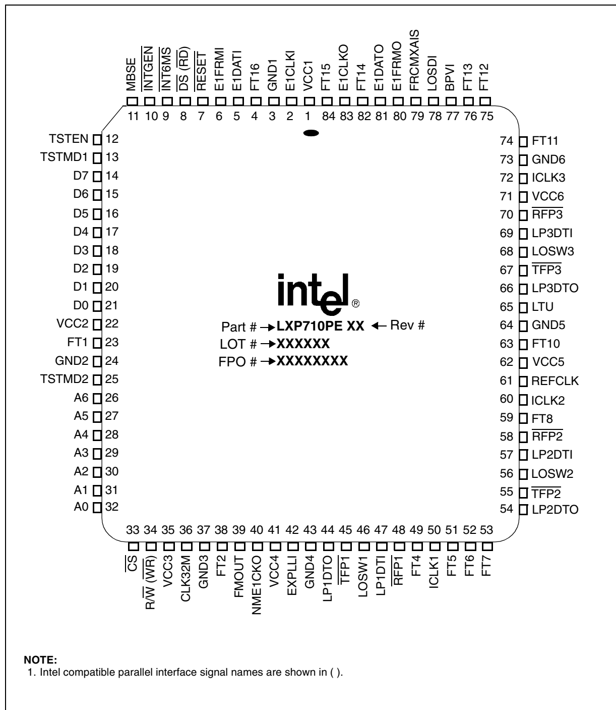
Figure 2. LXP710 Pinout Diagram
