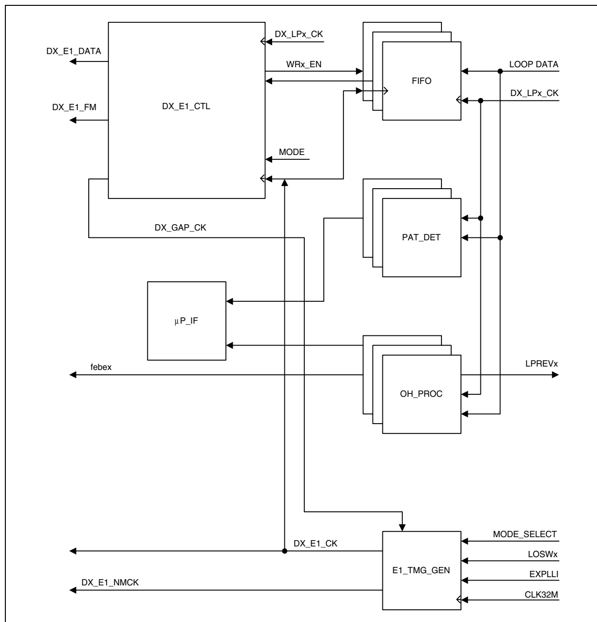
Figure 4. DX Process
