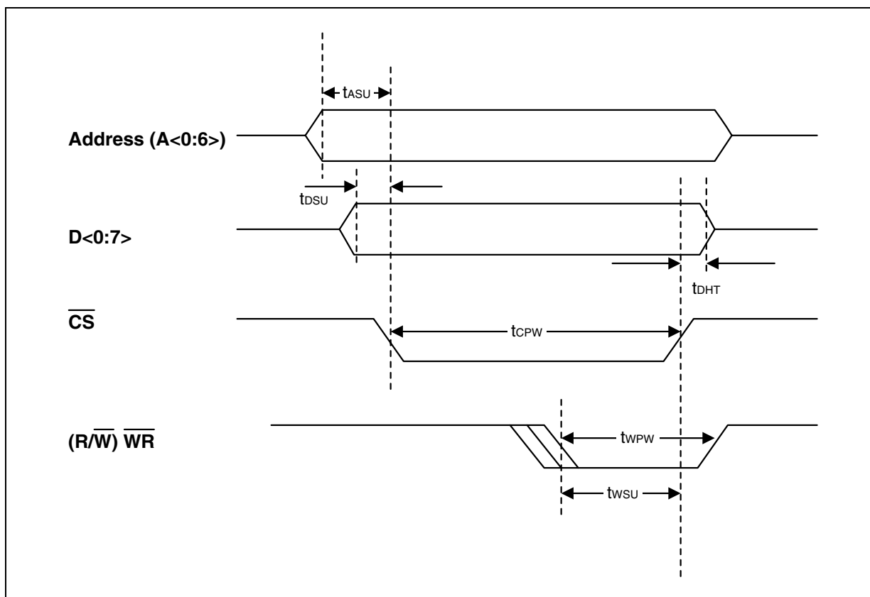
Figure 17. Microprocessor Write Cycle—Intel Mode
