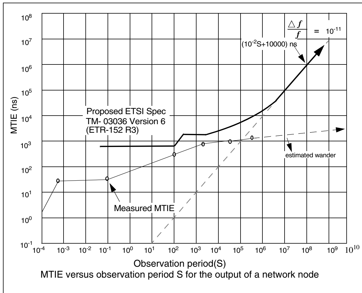
Figure 20. Output Wander Performance
