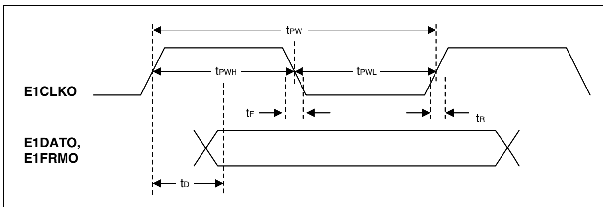
Figure 12. E1 Interface Output Timing
