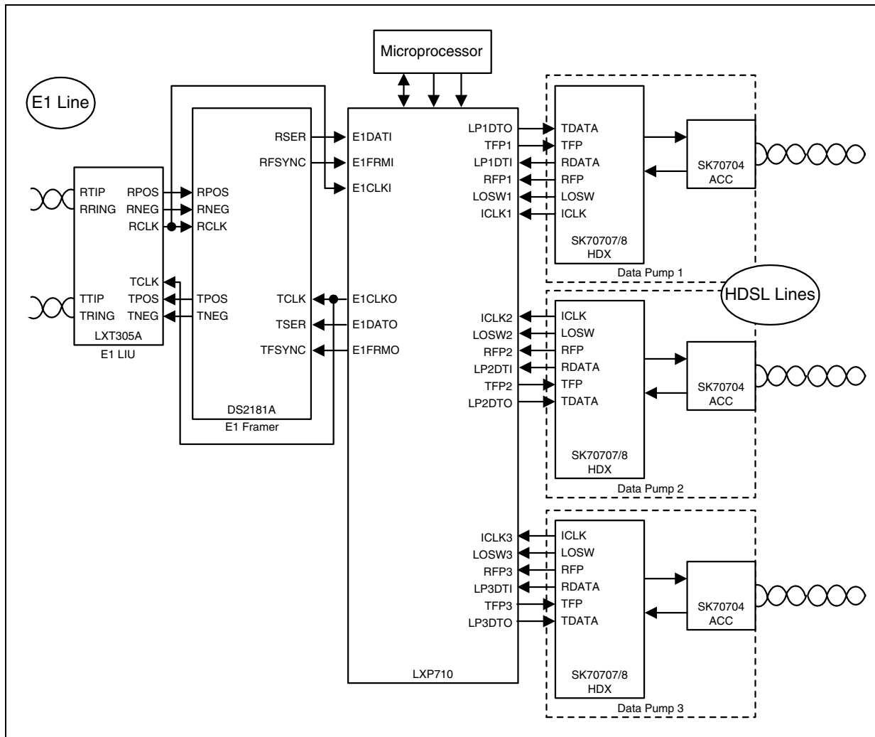
Figure 9. Point-to-Multipoint E1 HDSL System
