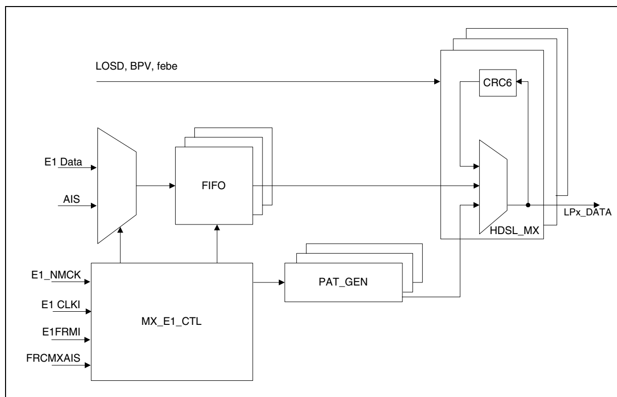
Figure 3. MX Process
