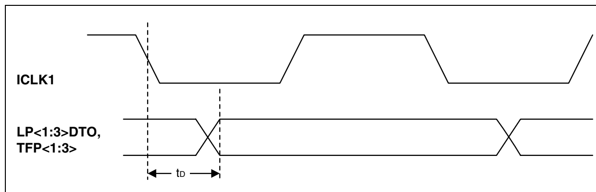
Figure 14. HDSL Interface Output Timing
