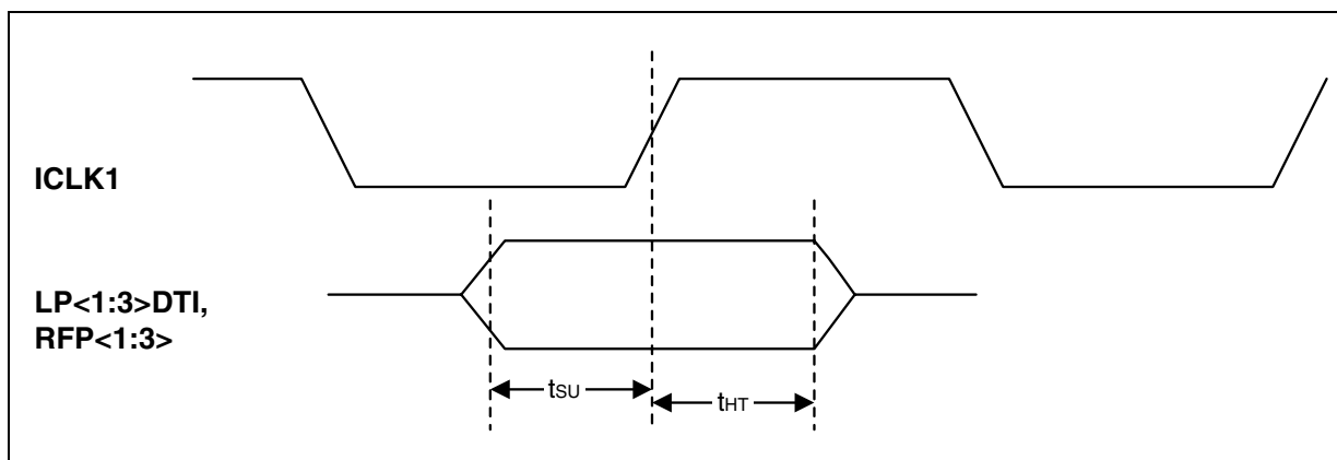
Figure 13. HDSL Interface Input Timing
