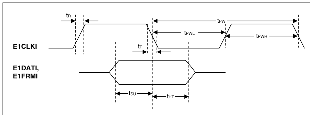
Figure 11. E1 Interface Input Timing
