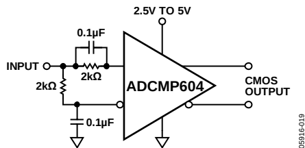
Figure 21. Self-Biased, 50% Slicer
