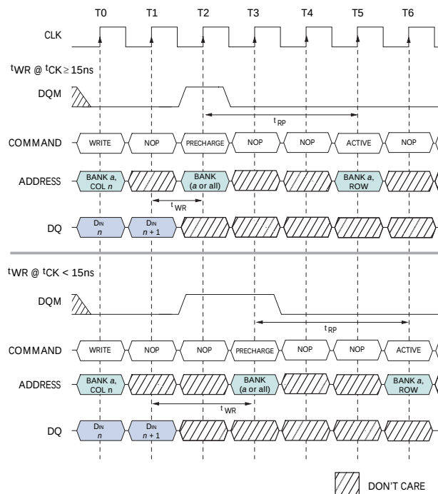
Figure 21: WRITE to PRECHARGE
