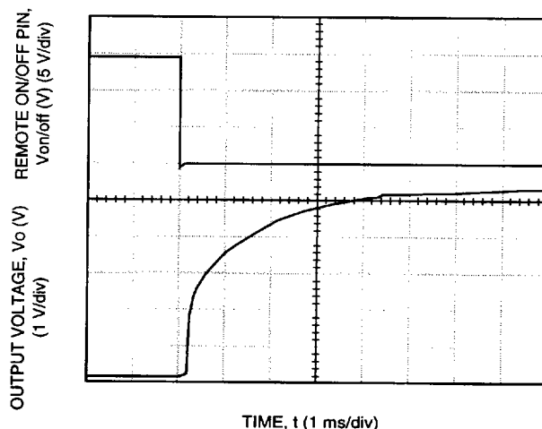
Figure 8. Typical FE150N Start-Up Transient at Room Temperature, 48 V Input, and 12.5 A Output
