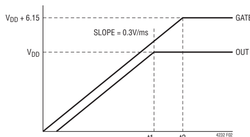
Figure 2. Supply Turn-On
