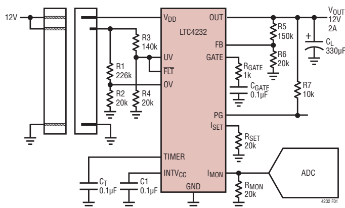
Figure 1. 2A, 12V Card Resident Application
