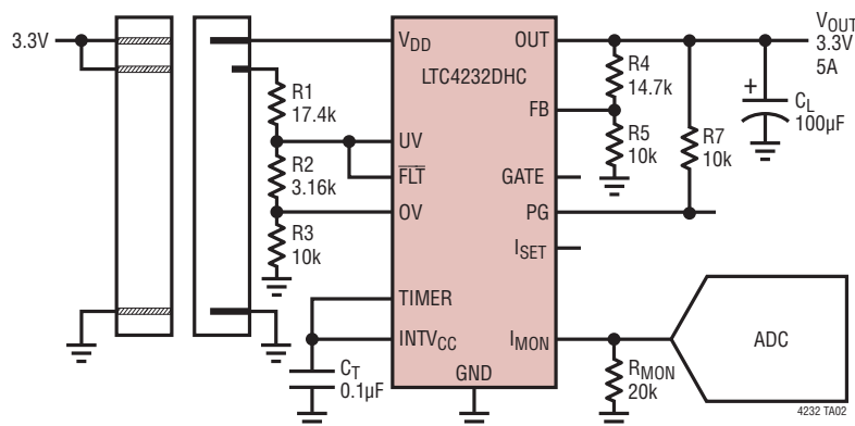
3.3V, 5A Card Resident Application with Auto-Retry
