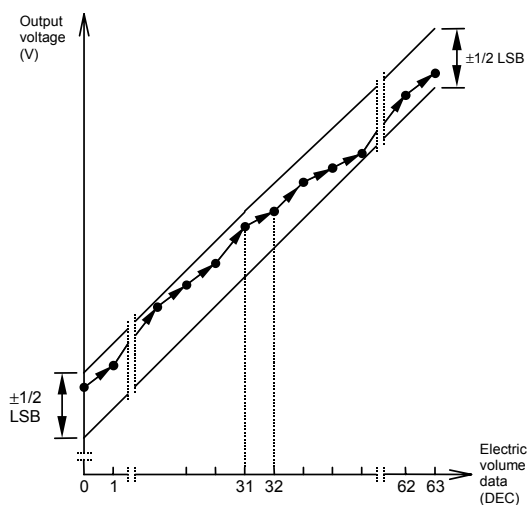
Figure 10 Linearity Error
