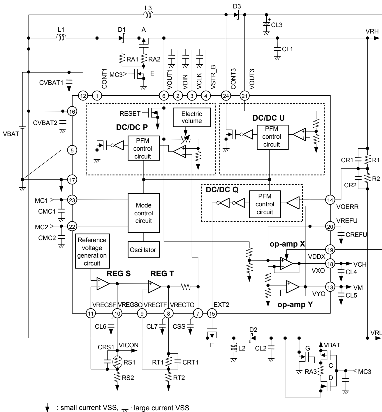
Figure 19 Standard Circuits
