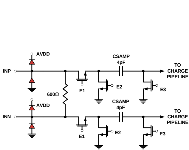
FIGURE 43. ANALOG INPUTS
