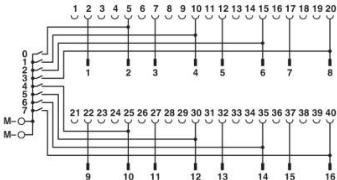
Connection scheme FLKM 16-PA-331-1KF//MINI-MCR
