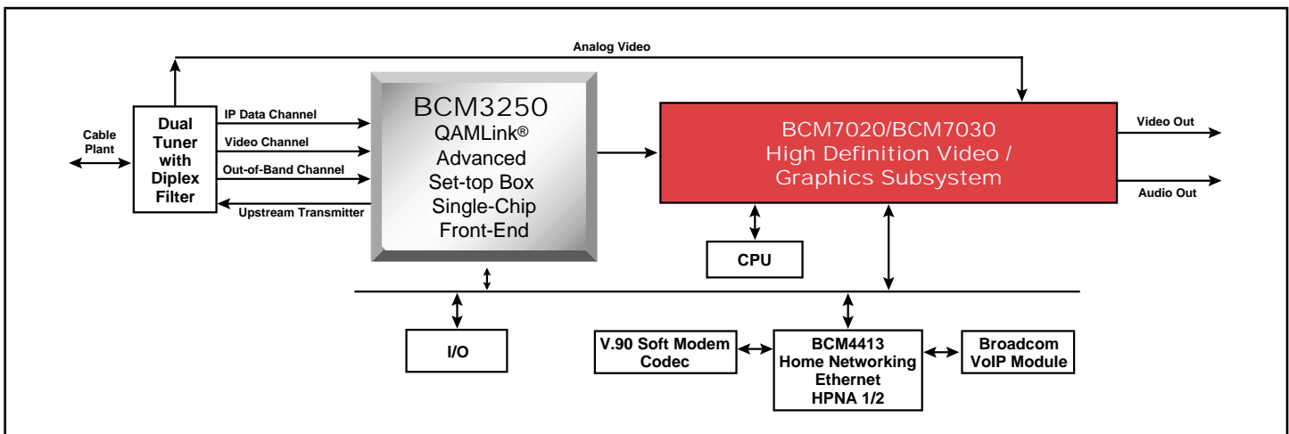
Interactive Set-top Box System Block Diagram
