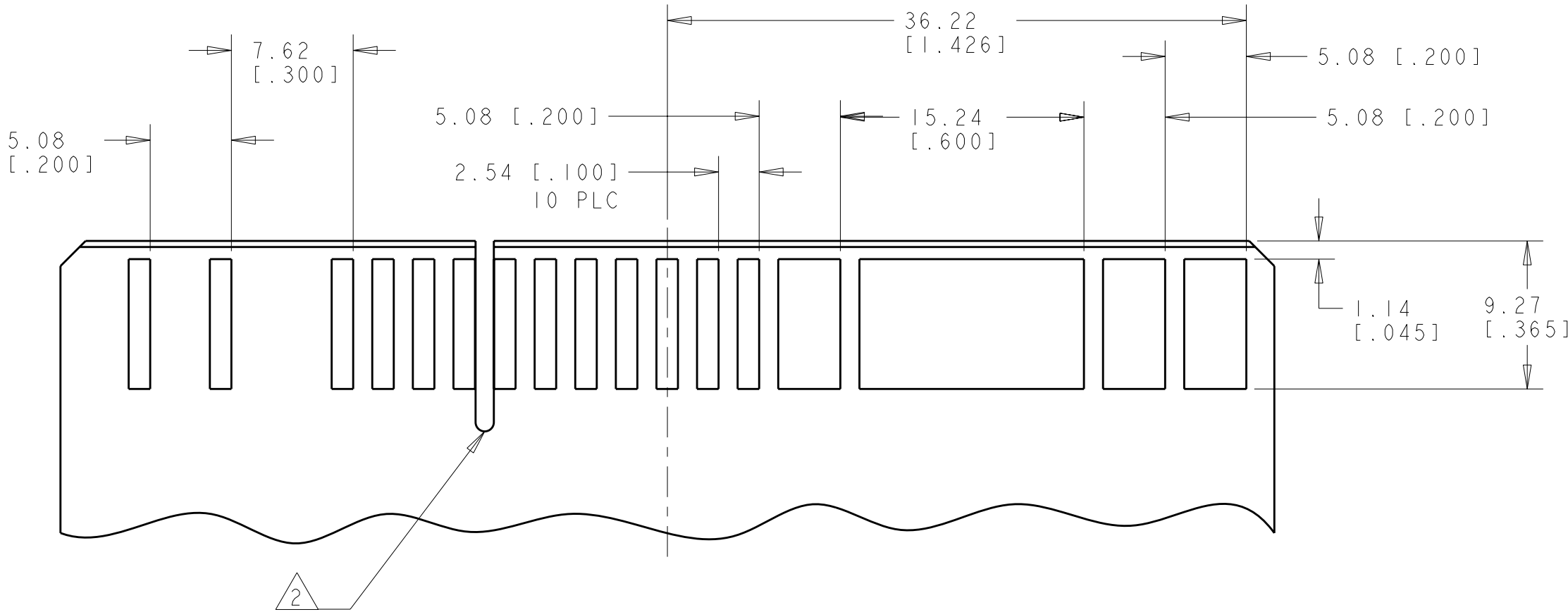
RECOMMENDED ETCHED CIRCUIT
