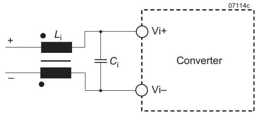
Fig. 14 External filter circuitry
