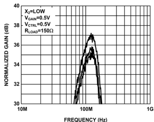
FIGURE 6. CHANNEL MISMATCH
