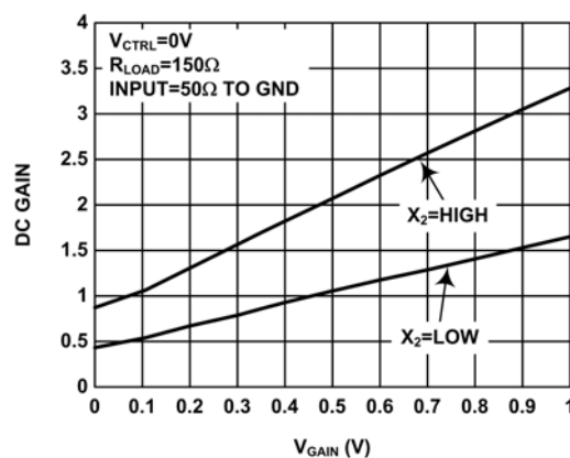
FIGURE 10. DC GAIN vs V_{GAIN}
