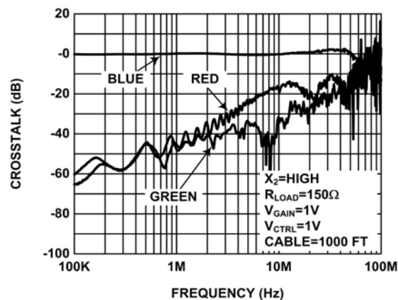
FIGURE 16. BLUE CROSSTALK
