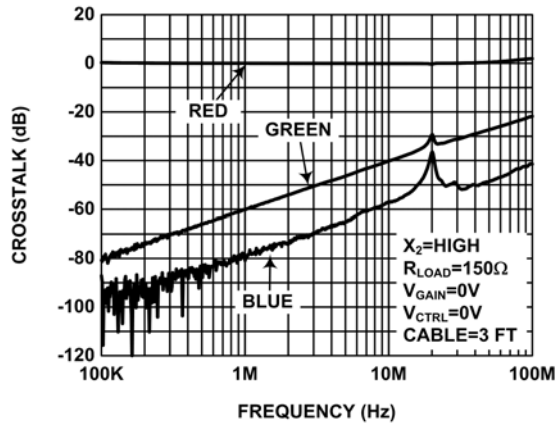
FIGURE 19. RED CROSSTALK
