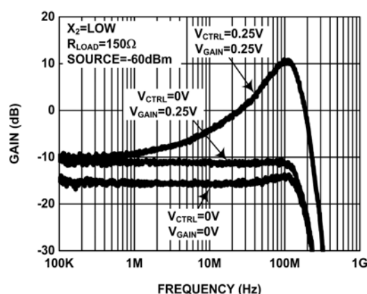
FIGURE 4. GAIN vs FREQUENCY FOR VARIOUS V CTRL AND V GAIN
