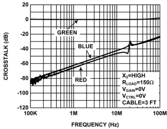
FIGURE 17. GREEN CROSSTALK
