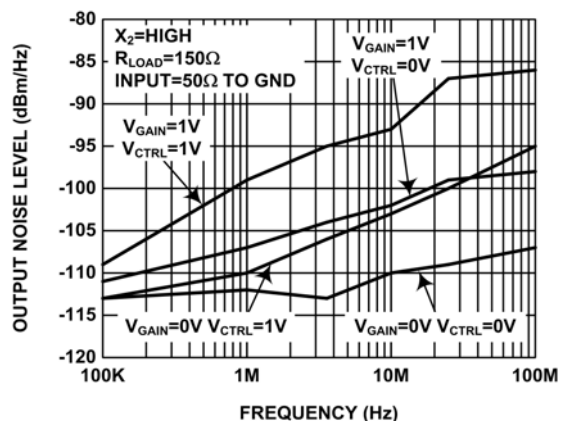
FIGURE 8. OUTPUT NOISE
