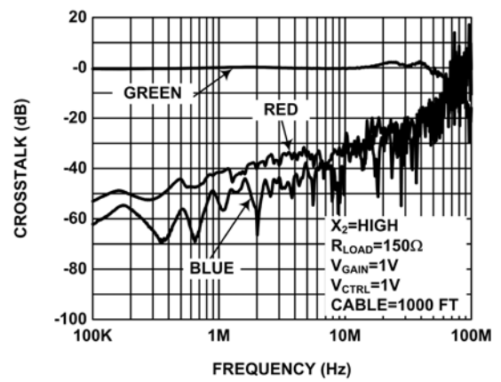
FIGURE 18. GREEN CROSSTALK
