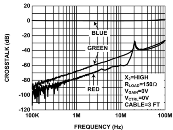
FIGURE 15. BLUE CROSSTALK
