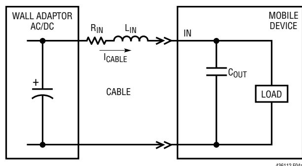
Figure 4. 20V Hot-Plug into a 10 \mu F Capacitor
