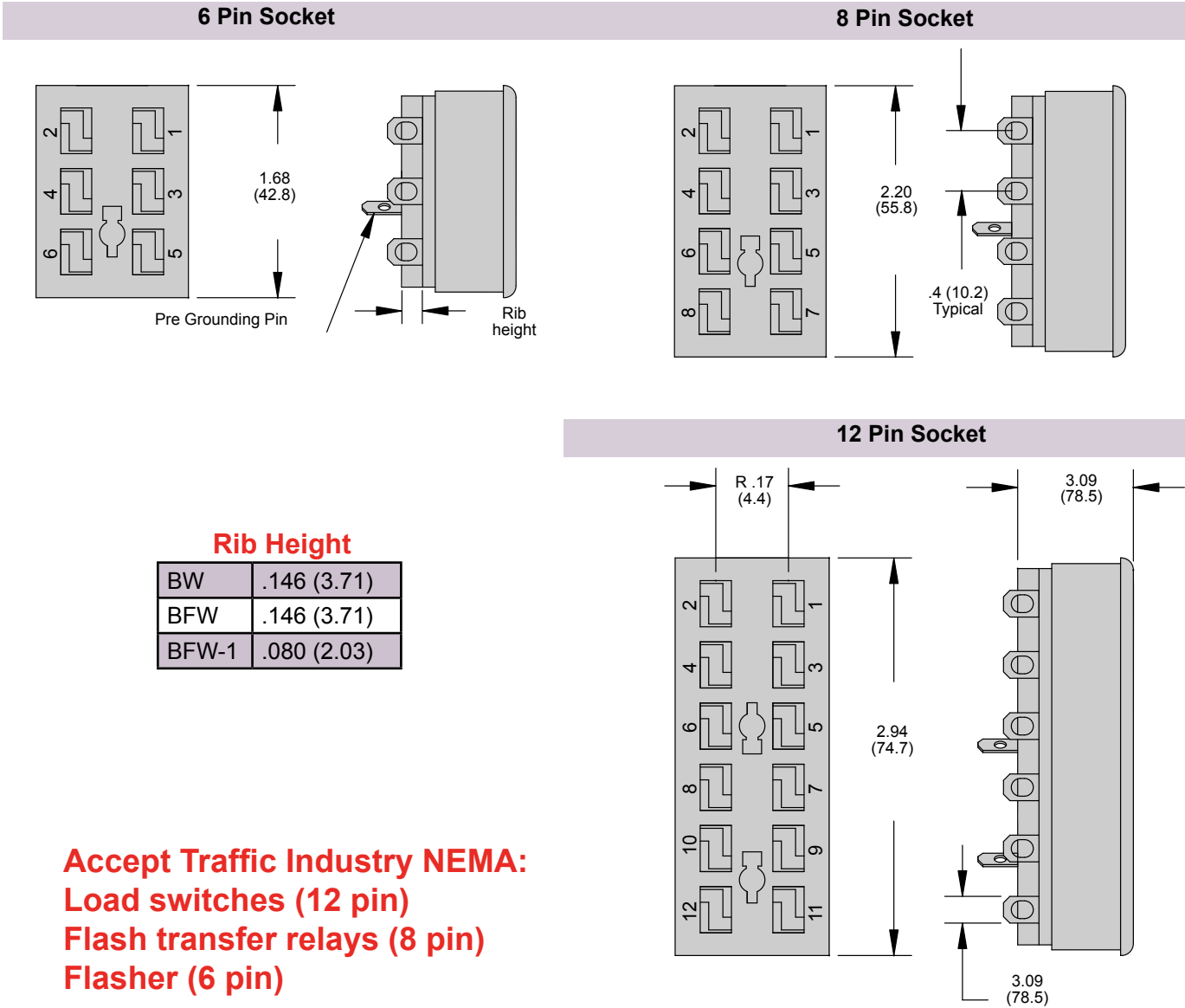
Outline Dimensions Dimensions Shown in inches & (millimeters)
