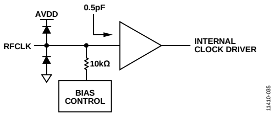
Figure 34. Equivalent Clock Input Circuit
