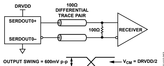
Figure 63. DC-Coupled Digital Output Termination Example
