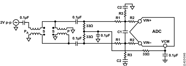
Figure 46. Differential Double Balun Input Configuration
