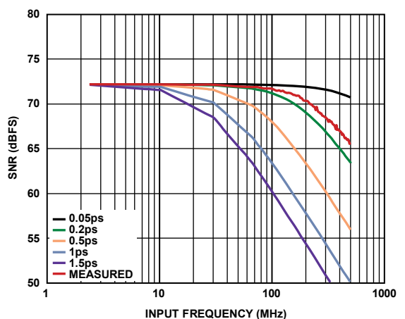
Figure 57. AD9683-250 SNR vs. Input Frequency and Jitter
