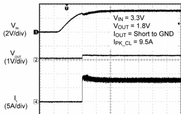
Power Up into Short Circuit
