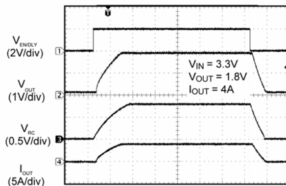
Enable Turn-On/Turn-Off
