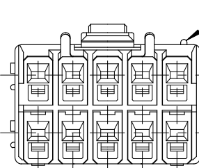
SHAPE OF 51284-1001
