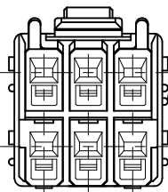
SHAPE OF 51284-0600
