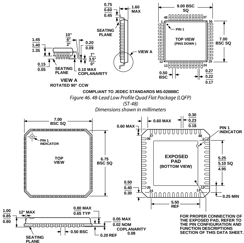
COMPLIANT TO JEDEC STANDARDS MO-220-VKGD-2 Figure 47. 48-Lead Lead Frame Chip Scale Package [LFCSP_VQ] 7 × 7 mm Body, Very Thin Quad (CP-48-1)
