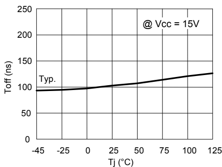
Figure 9. Turn-off time vs. temperature
