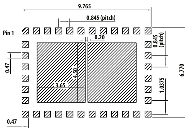
Stencil Opening
