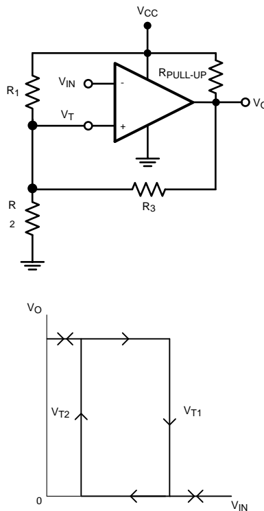
Figure 10. Inverting Configured Comparator - LM397
