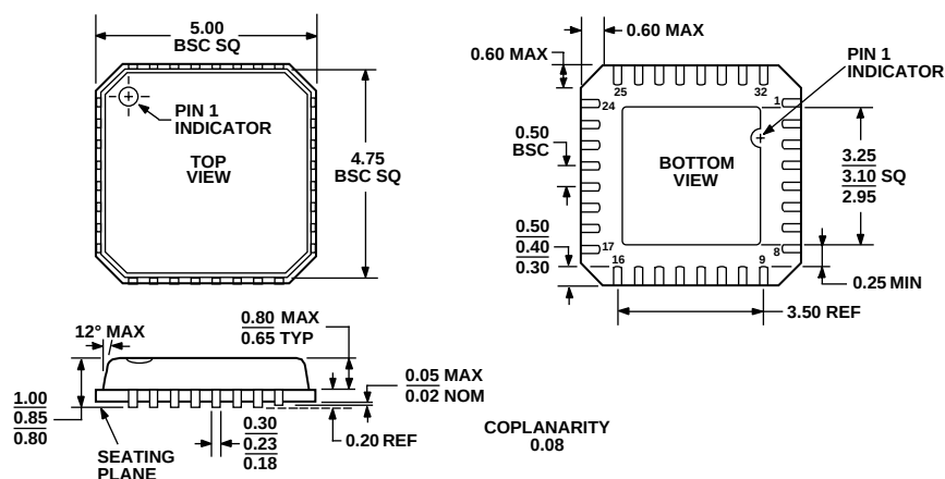
Figure 42. 32-Lead Lead Frame Chip Scale Package [LFCSP] 5 mm x 5 mm Body (CP-32-2)
