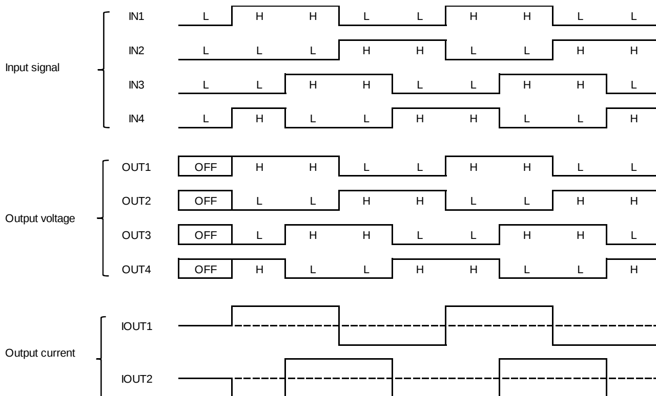
2 phase excitation timing chart
