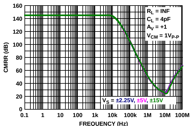
FIGURE 37. CMRR vs FREQUENCY, V_S = \pm 2.25 , \pm 5V , \pm 15V
