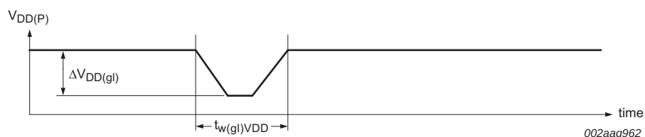
Fig 17. Glitch width and glitch height
