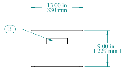
R.S. VIEW
