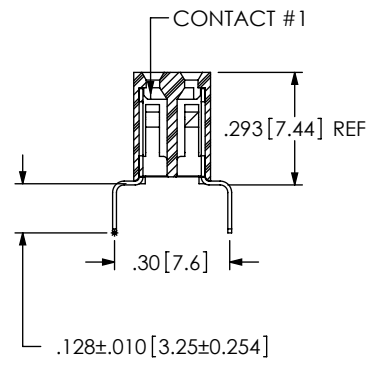
FIG 4 -PE/-PE-BE (SEE SHEET 3 FOR IN-PROCESS)
