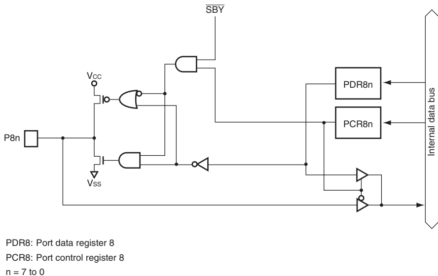
Figure B.7 Port 8 Block Diagram
