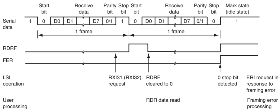
Figure 15.7 Example SCI3 Operation in Reception in Asynchronous Mode (8-Bit Data, Parity, One Stop Bit)
