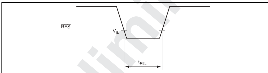
Figure 24.3 \overline{RES} Low Width Timing
