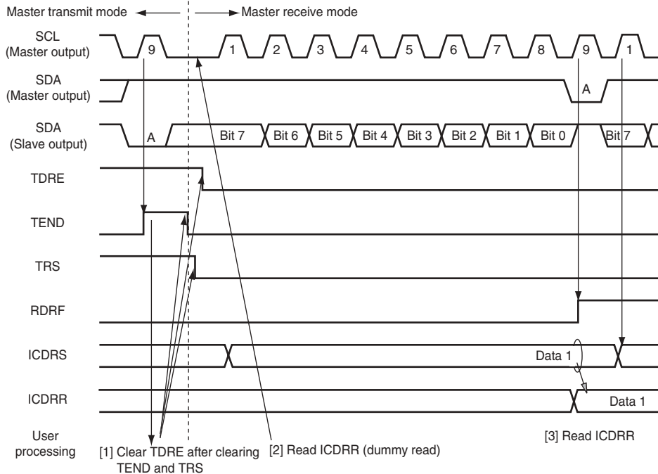
Figure 20.7 Master Receive Mode Operation Timing (1)
