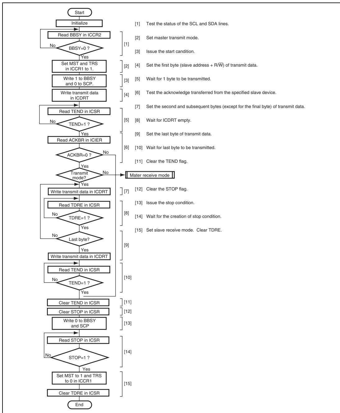
Figure 20.17 Sample Flowchart for Master Transmit Mode
