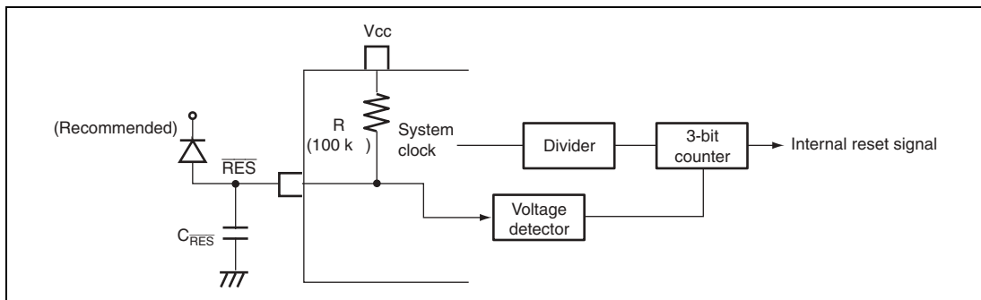
Figure 21.1 Power-On Reset Circuit
