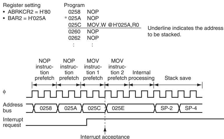
Figure 22.2 Address Break Interrupt Operation Example (1)
