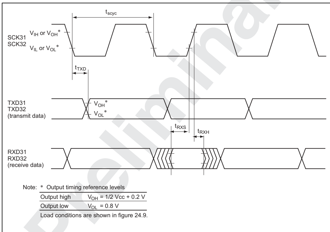
Figure 24.6 SCI3 Input/Output Timing in Clocked Synchronous Mode
