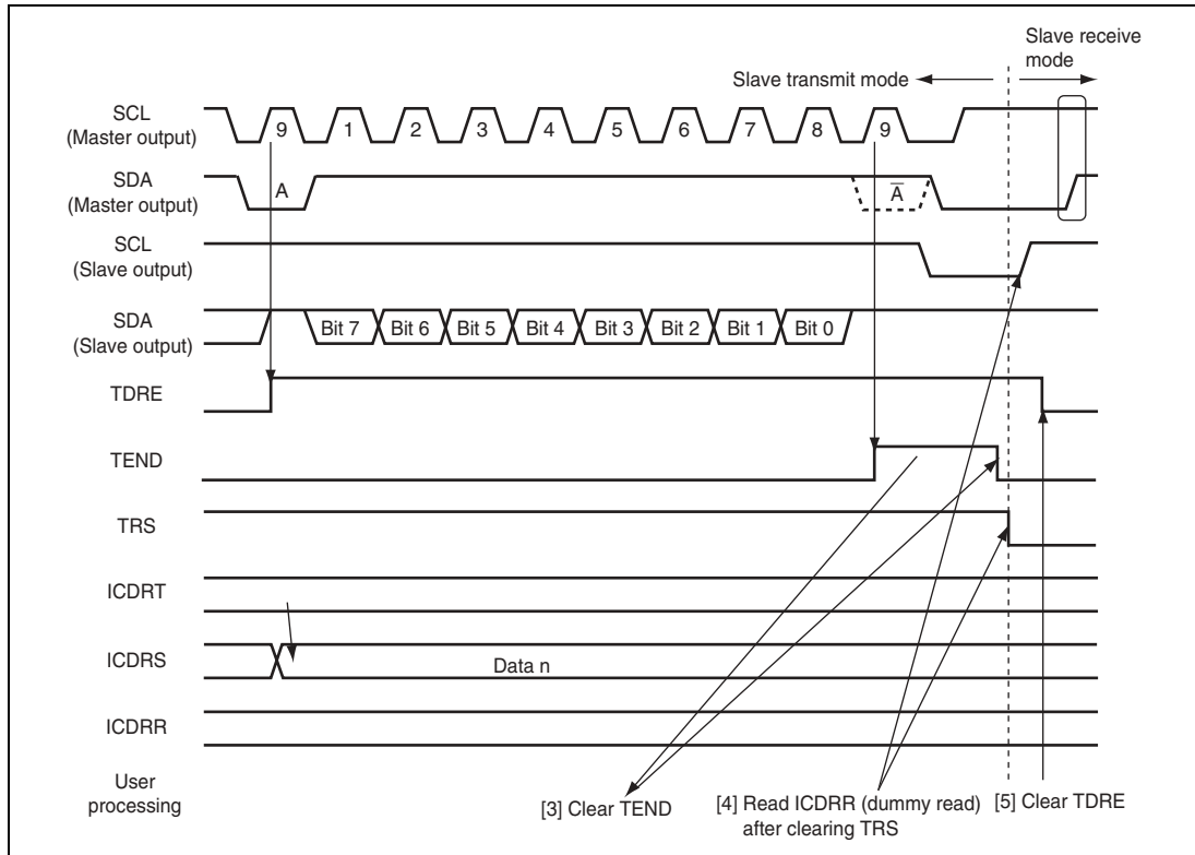
Figure 20.10 Slave Transmit Mode Operation Timing (2)
