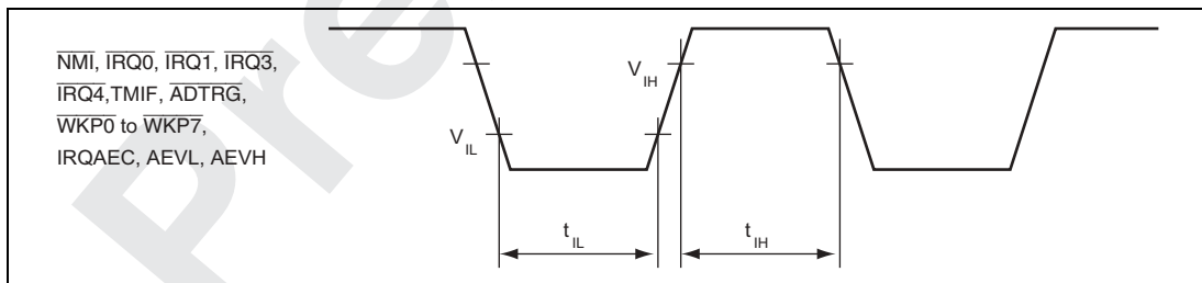
Figure 24.4 Input Timing
