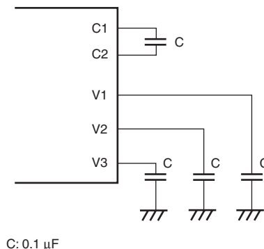
Figure 19.9 Capacitance Connection when Using 3-V Constant-Voltage Power Supply Circuit
