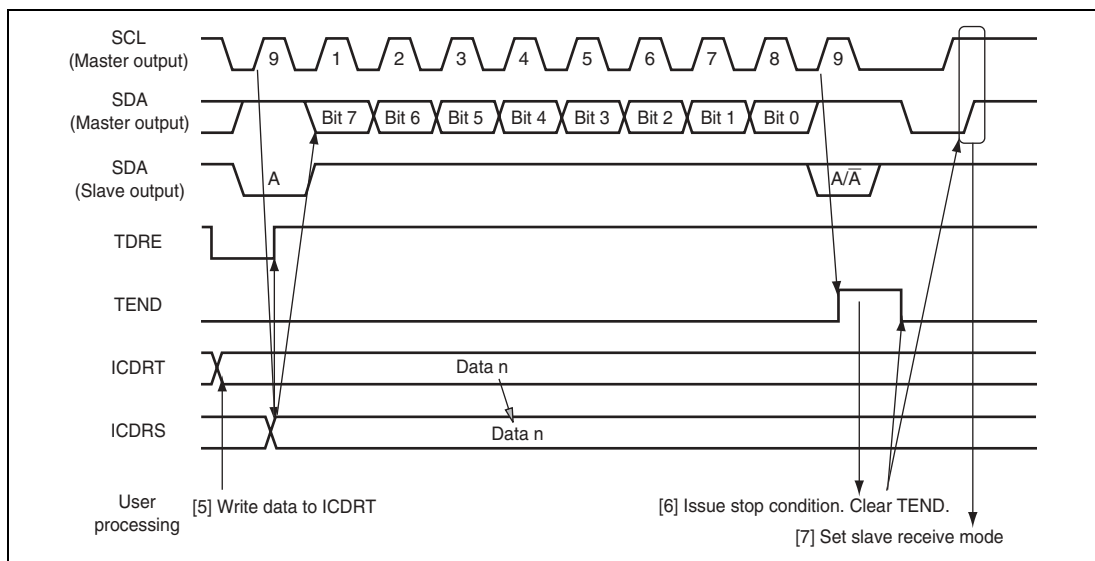
Figure 20.6 Master Transmit Mode Operation Timing (2)
