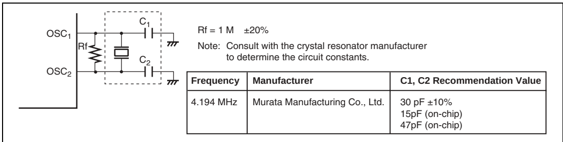
Figure 5.4 Typical Connection to Ceramic Resonator
