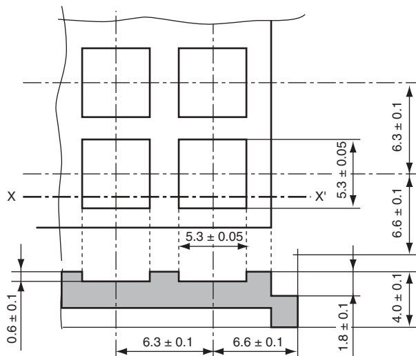
Figure G.2 Chip Tray Specifications (HCD64F38076R)
