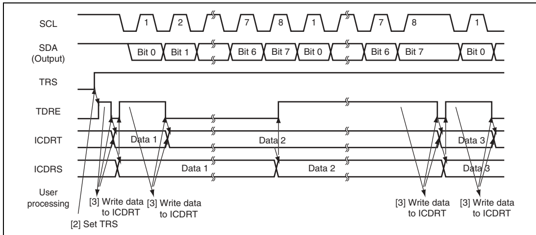
Figure 20.14 Transmit Mode Operation Timing
