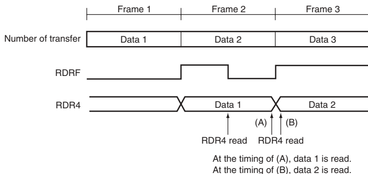
Figure 16.9 Relationship between Reading RDR4 and RDRF
