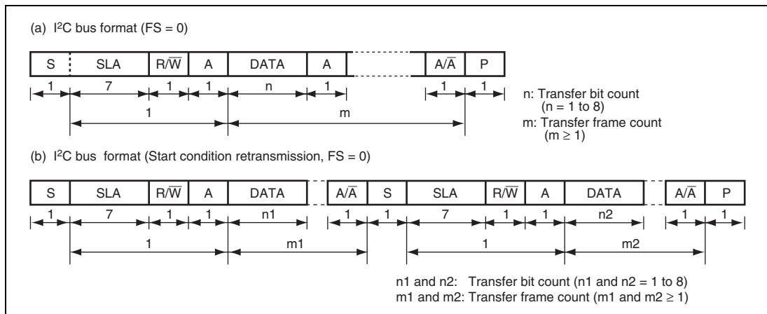
Figure 20.3 I 2 C Bus Formats
