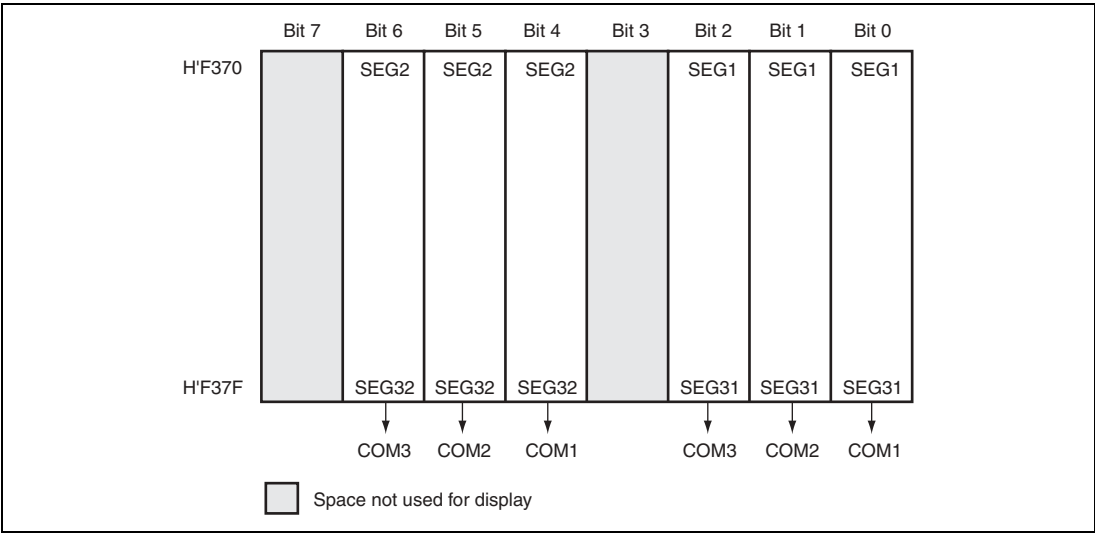
Figure 19.4 LCD RAM Map (1/3 Duty)
