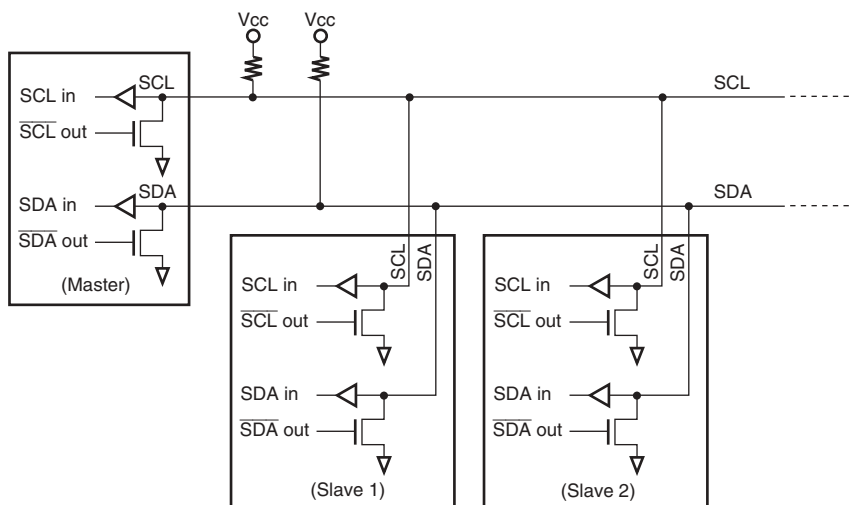
Figure 20.2 External Circuit Connections of I/O Pins
