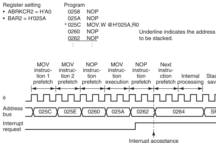
Figure 22.2 Address Break Interrupt Operation Example (2)
