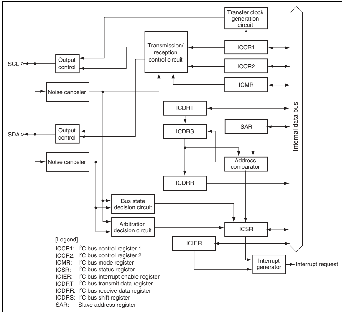
Figure 20.1 Block Diagram of I²C Bus Interface 2
