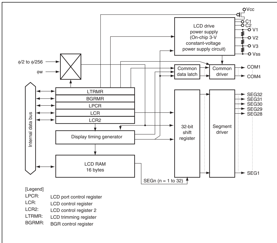
Figure 19.1 Block Diagram of LCD Controller/Driver
