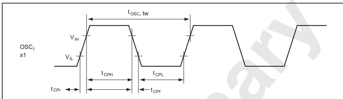
Figure 24.2 Clock Input Timing
