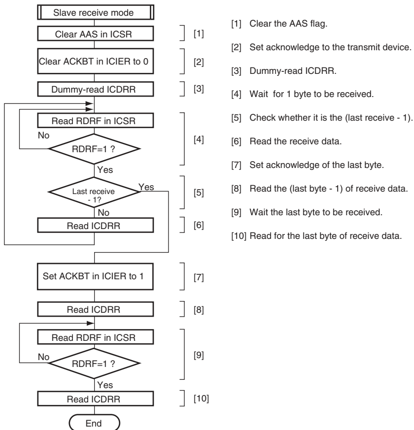
Figure 20.20 Sample Flowchart for Slave Receive Mode
