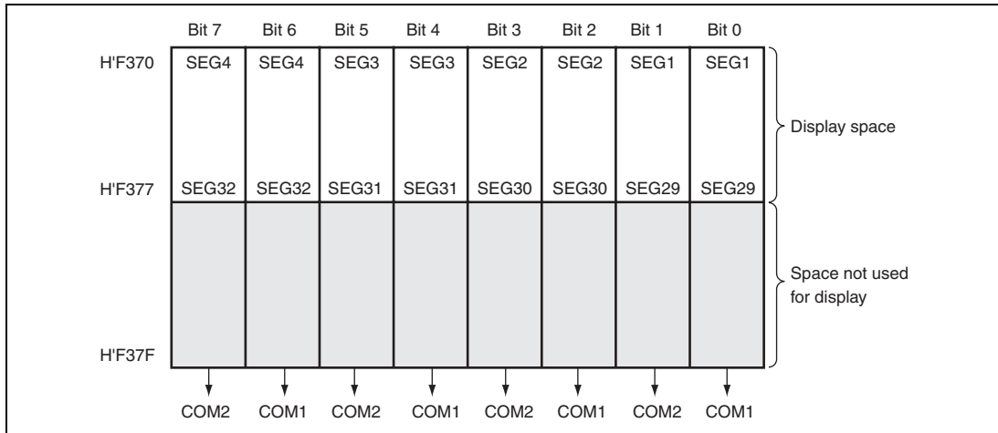
Figure 19.5 LCD RAM Map (1/2 Duty)
