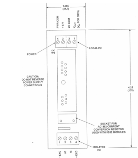
Figure 4 Outline Dimensions 5B03
