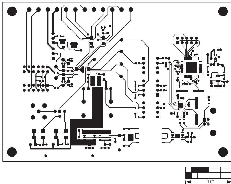
Figure 10. MAX11200/MAX11206/MAX11209/MAX11210/MAX11213 EV Kit PCB Layout—Component Side
