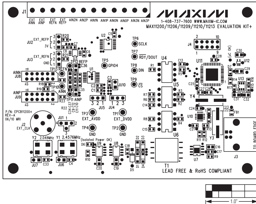
Figure 9. MAX11200/MAX11206/MAX11209/MAX11210/MAX11213 EV Kit Component Placement Guide—Component Side
