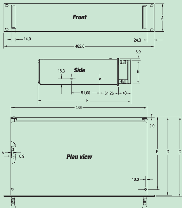
19" Rack cases
