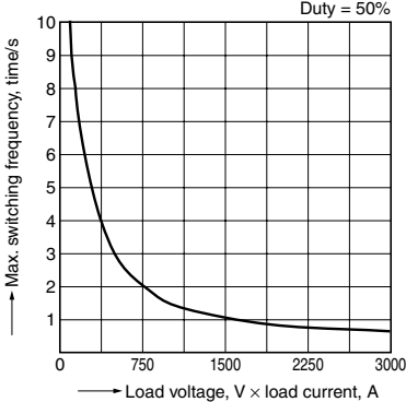
2. Max. switching frequency vs. load voltage × load current characteristics Ambient temperature: 20°C 68°F
